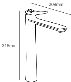
Miscelatore lavabo alto Sleeve wash basin mixer
