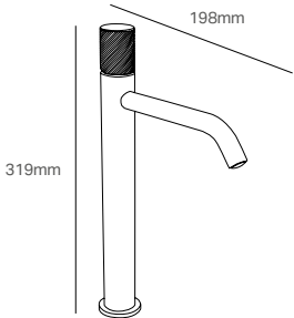
Miscelatore lavabo alto Sleeve wash basin mixer
